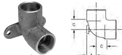
707-5 90° Drop Elbow C x C – Cast
