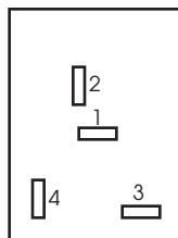
Terminal Layout (bottom view)
