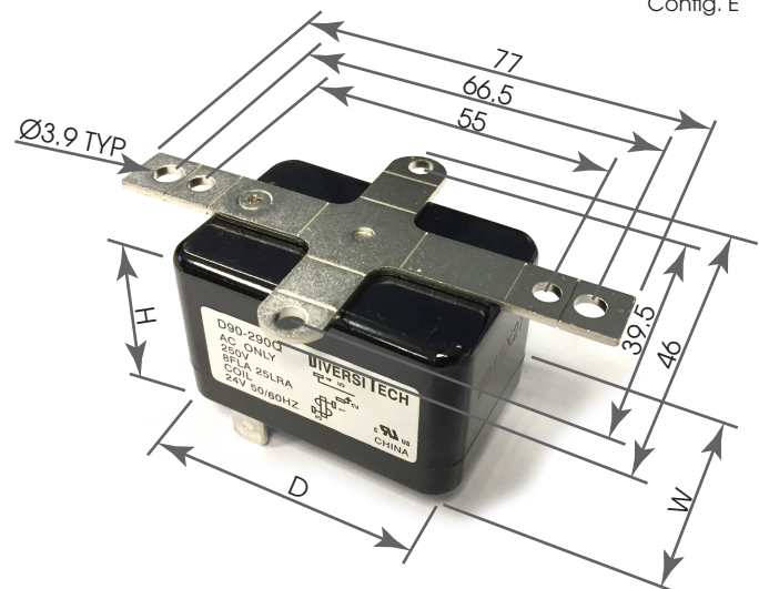
Overall Dimensions (mm)
