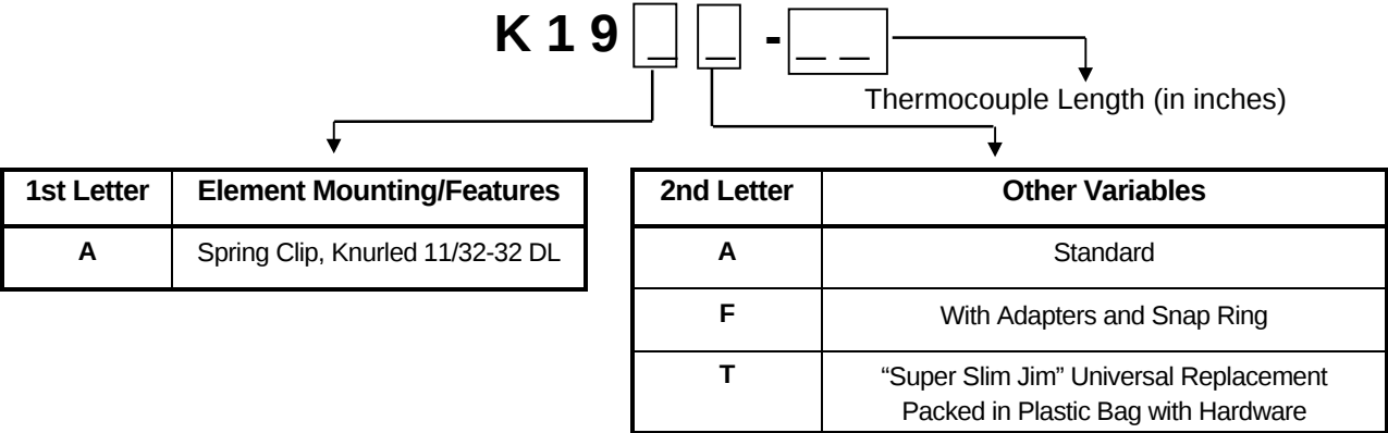
Figure 8: K19 Thermocouple
