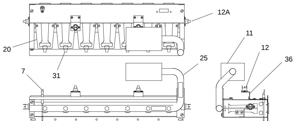
Figure 3: GAS CONTROLS
