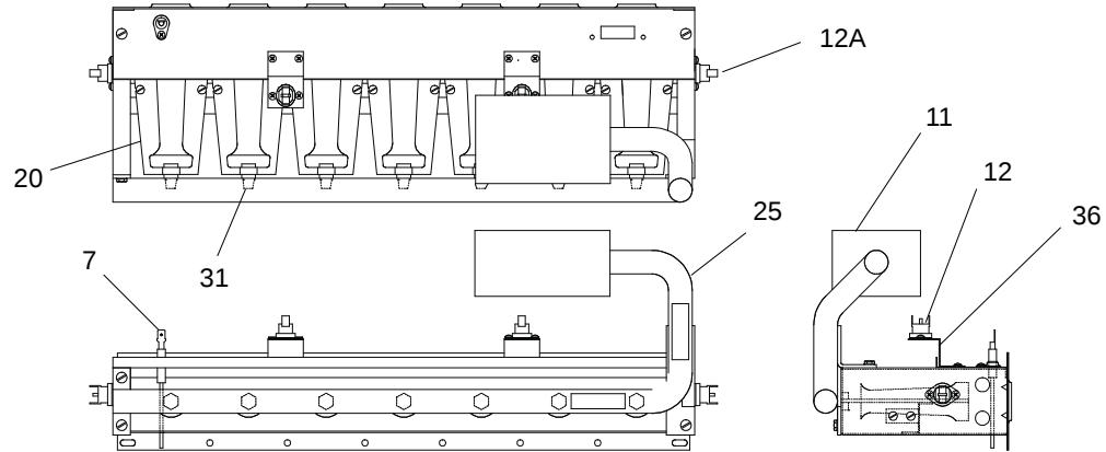
Figure 3: GAS CONTROLS
