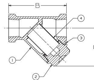
T-221/222-B Threaded
