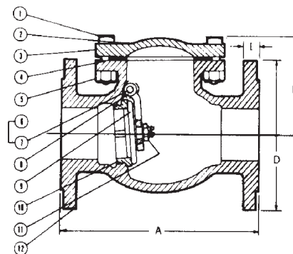
F-938-33
