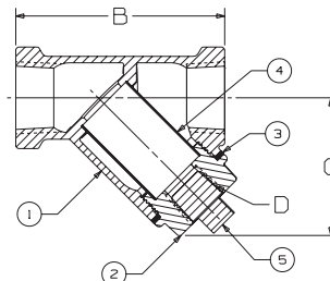
T-221/222-A Threaded
