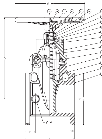
F-619-RWS
